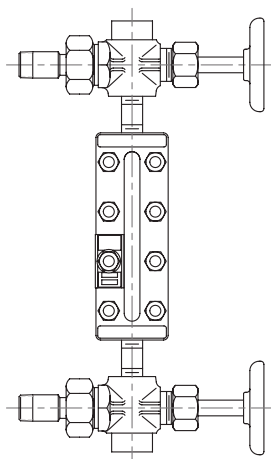
END CONNECTED GAUGE W/GAUGECOCKS
