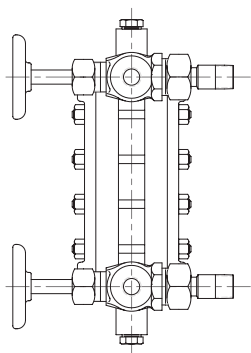
SIDE CONNECTED GAUGE W/GAUGECOCKS
